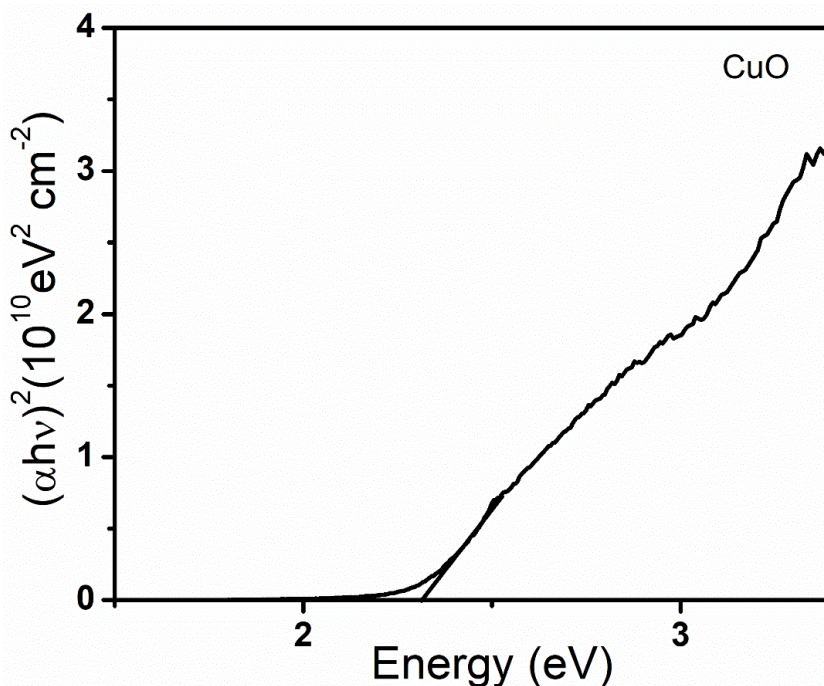
Figure 4. Tauc's plot of pure CuO
