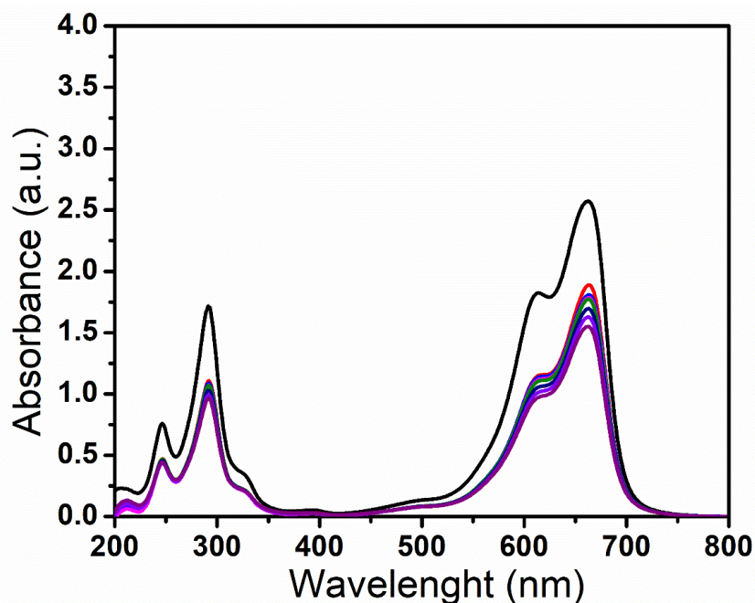
Figure 5. UV-vis absorbance spectra of MB dye solution
