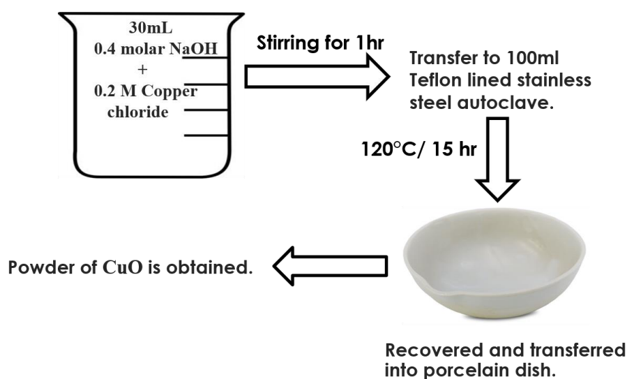
Figure 1. Synthesis route of CuO Nano powders
